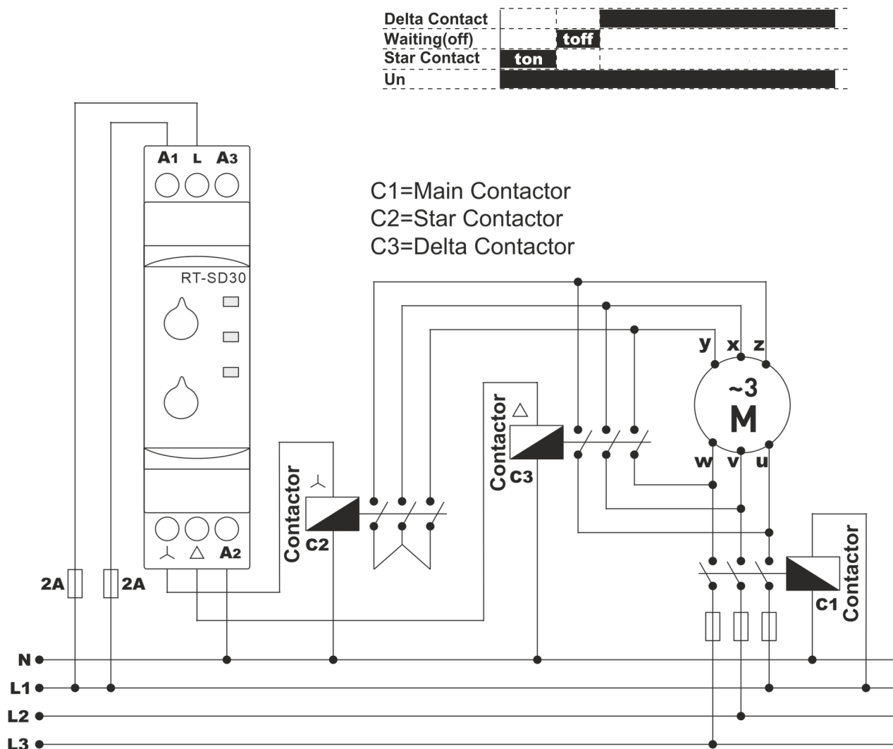
Connection diagram for RT-SD30-U
