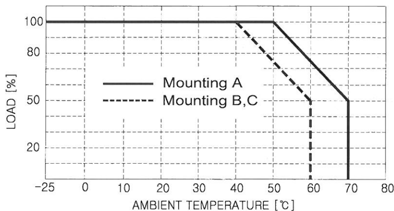
< Fig.11 Output Derating Curve >
