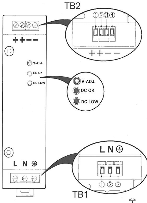
TB1 : Input Terminal Assignment
