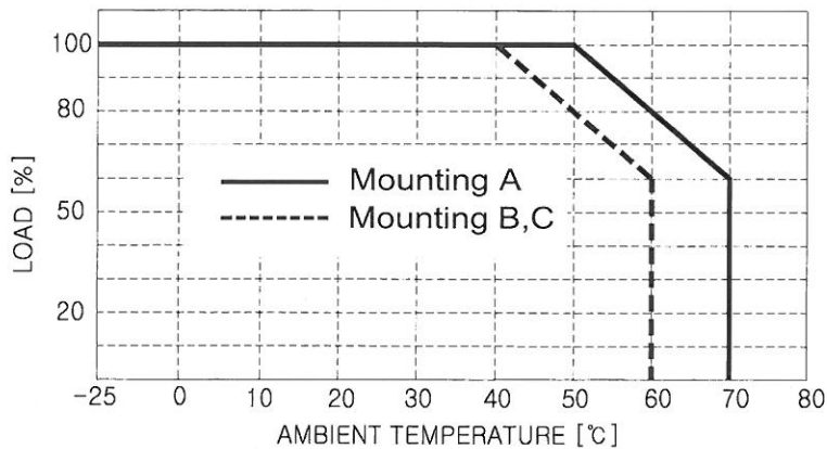
< Fig.11 Output Derating Curve >
