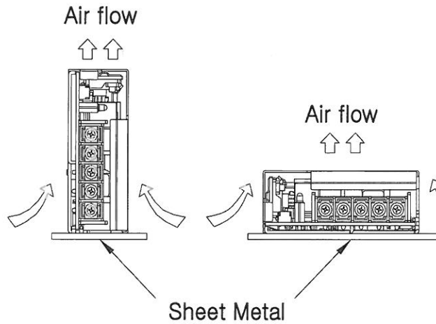
(1) MOUNT A
