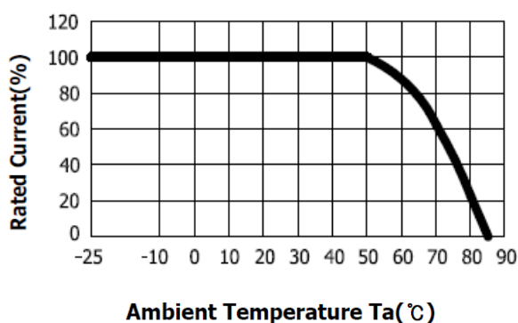
- Derating Curve
