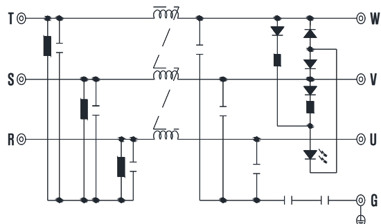
- Circuit Diagram
