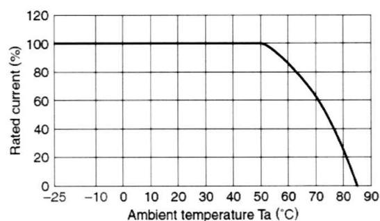
- Derating Curve
