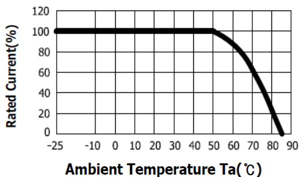
- Derating Curve
