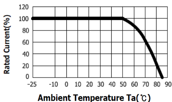
- Derating Curve
