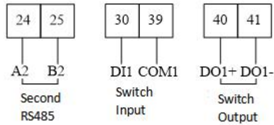
Fig 11 Communication, pulse connection
