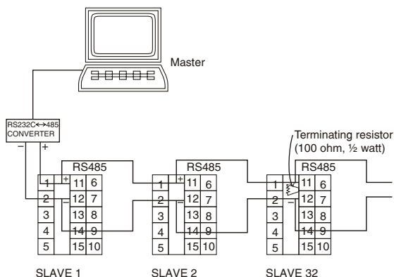
CONNECTION DIAGRAM
