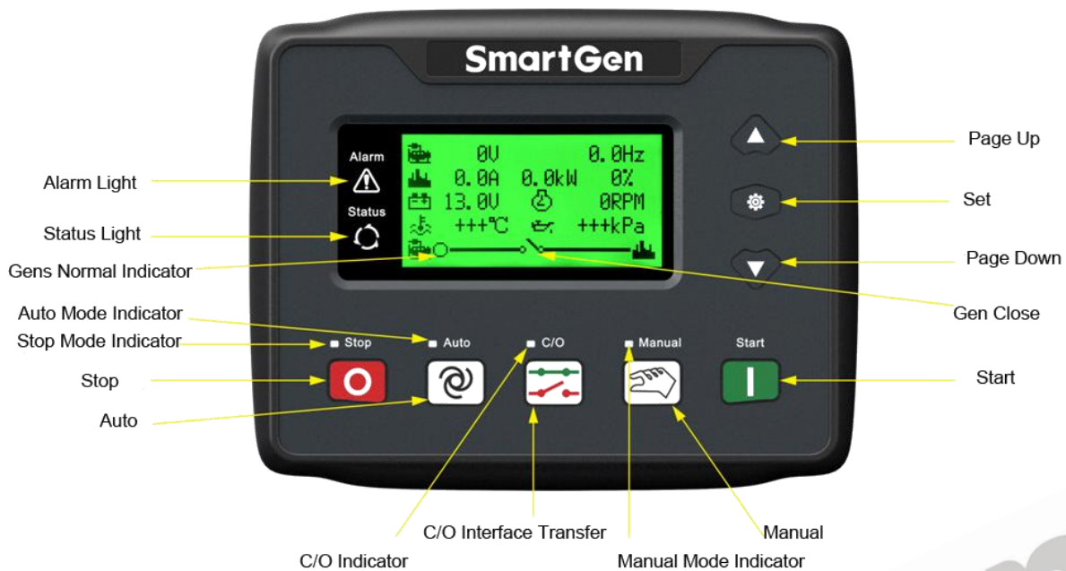
Fig.1 - HGM4010N/HGM4010NC/HGM4010CAN Front Panel Indication
