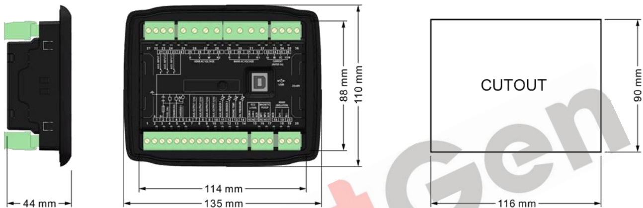
Fig.10 - Overall Dimensions
