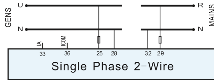
Fig.8 - Single Phase 2-Wire Connection Diagram
